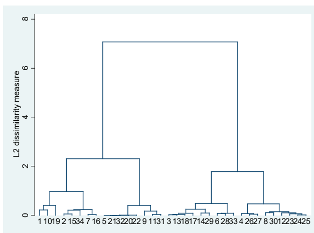
Graph 1. Dendrogram for R&D clusters
