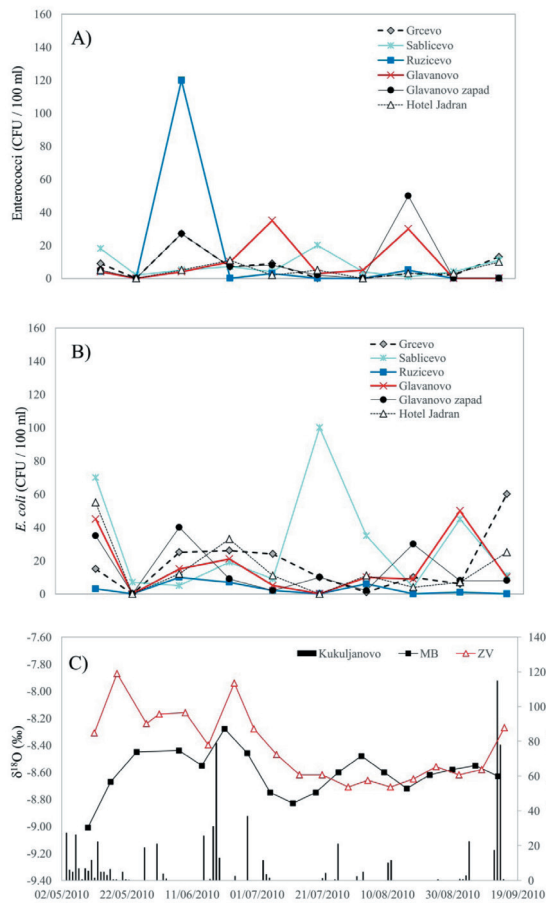
Fig. 6. Pećine, bathing season 2010: A) enterococci; B) E. coli ; C) daily precipitation amount at station Kukuljanovo and spring and well water \delta^{18}\text{O} time series. GR – Grčev; RZ – Ružičevo; GL – Glavanovo; GLW – Glavanovo west; SB – Sabličevo; HJ – beach at Hotel Jadran; MB – Martinšćica well; ZV – Zvir
